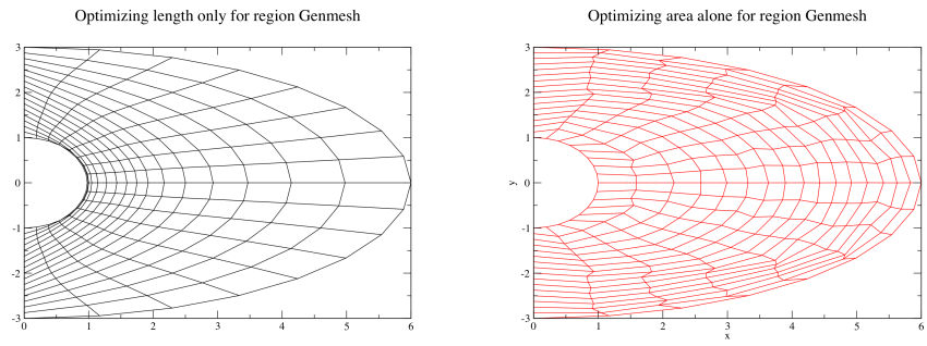
Figure 5: Problem Genmesh. Optimizing length and area separately.
