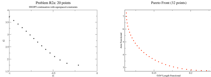
Figure 4: Results for problems R2a and Genmesh.
