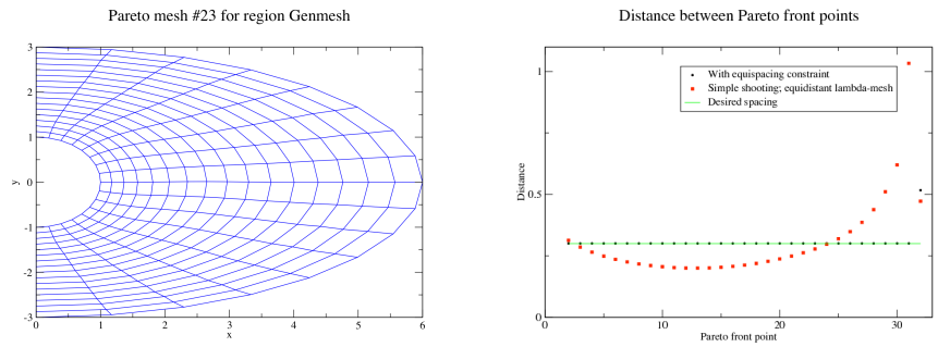
Figure 6: Problem Genmesh. Biobjective results.
