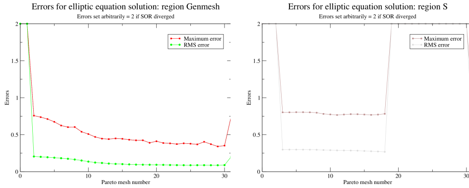
Figure 9: Errors for regions Genmesh and S.
