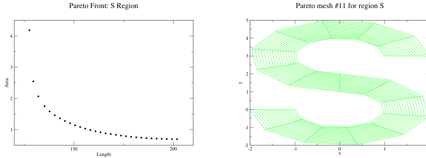
Figure 8: Pareto front for region S.
