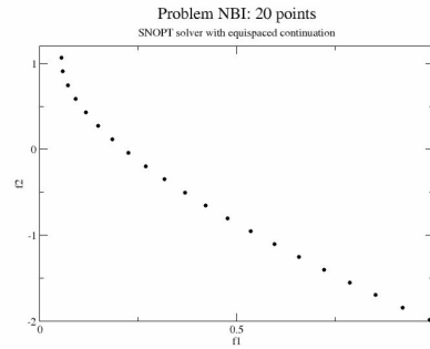
Figure 3: Pareto fronts for problems SRN and NBI.
