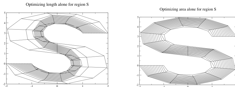
Figure 7: Problem S: Optimizing length and area separately.
