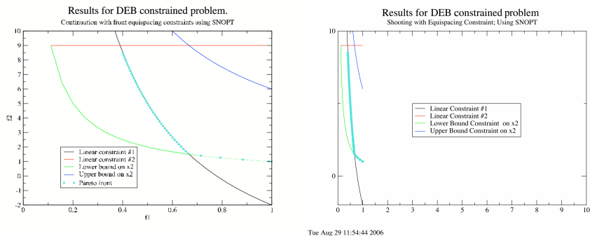
Figure 1: Results for problem DEB.
