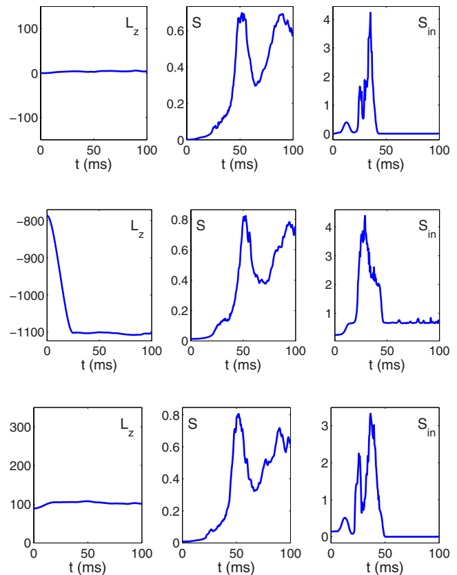
FIG. 6. (Color online) Vorticity indicators for the cases depicted in Fig. 5 (the different panels are presented in the same manner as in Fig. 4).
