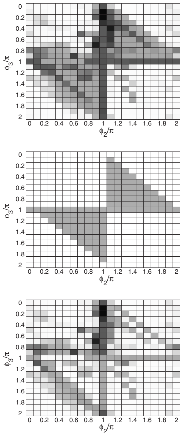
FIG. 7. Phase diagram for vortex formation at the trap center region as a function of the relative phases of the merging fragments (where \phi_1 is assigned the value of 0). Top: Ramp down time of t_b=0 ms (i.e., instantaneous removal) of the barrier. The different shades of gray indicate the amount of vorticity contained in the central region after 100 ms. White, light gray, gray, black correspond, respectively, to 0, 1, 2, and 3 vortices. Middle: Same as above for a ramp down time of t_b=50 ms. This case only produces no vortices (white) or one vortex (gray). Bottom: difference between top and middle diagrams. This corresponds to the vortices formed by the collision of the fragments and not by the intrinsic vorticity of the initial configuration (which depends on the relative phases of the different fragments).
